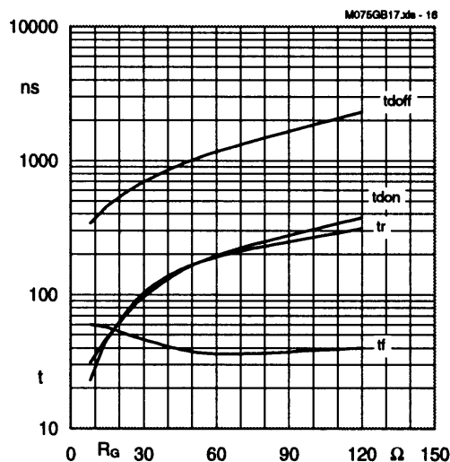
Fig. 16 Typ. switching times vs. R_G
